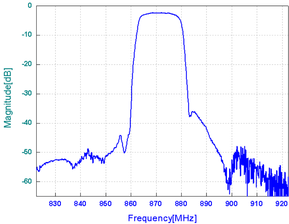
Frequency Response
